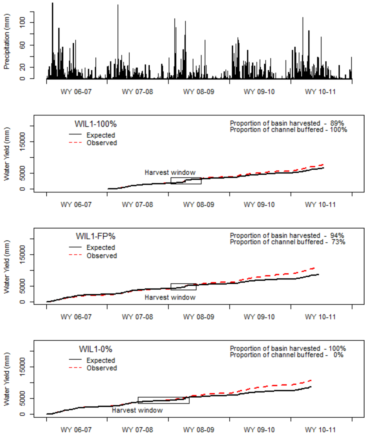
Figure 8-8. Precipitation at Aberdeen, Washington from October 1, 2006 to September 30, 2011 and cumulative water yield for the Willapa-1 block sites by water year (WY).
