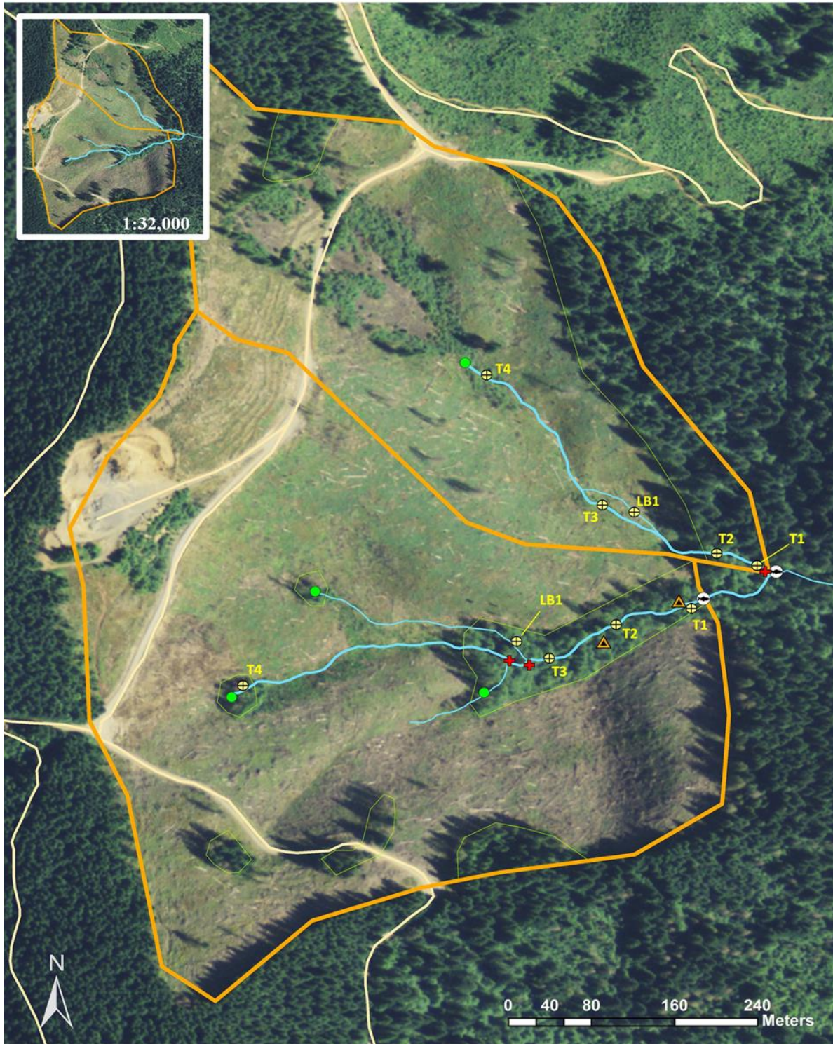
Appendix Figure 7-A-7. Monitoring locations in CASC-FP (lower) and CASC-0% (upper) sites.
