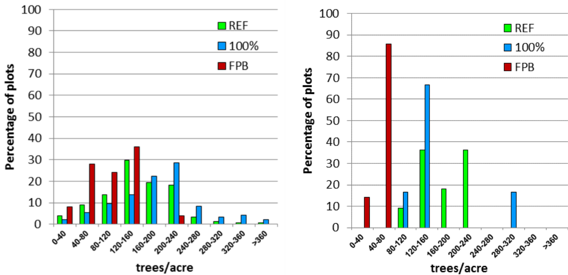
Figure 5-11. Distributions of RMZ (left panel) and PIP (right panel) plot values for live tree density (trees/ac) by experimental treatment, two years after harvest.
