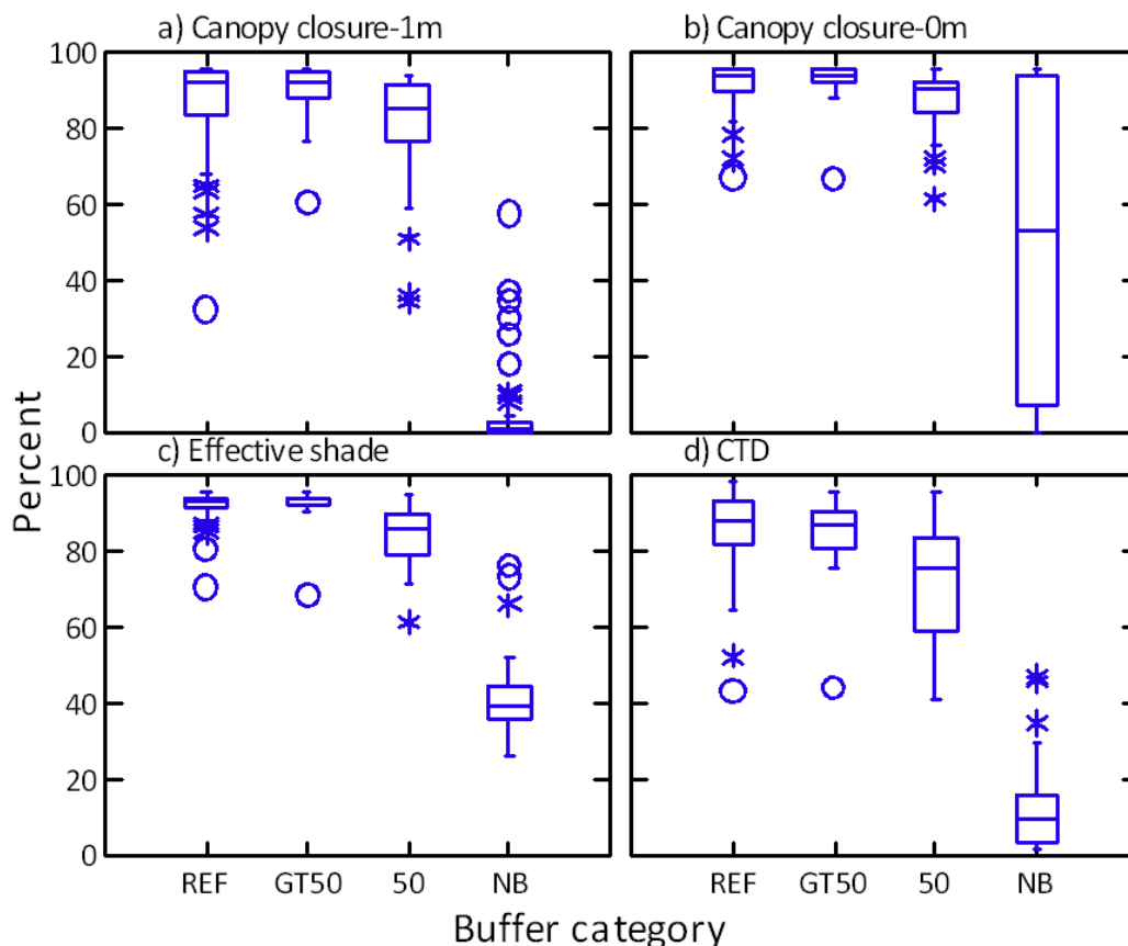
Figure 7-11. Distribution of post-harvest shade values by buffer width category. REF = reference site, GT50 = buffer greater than 50 ft (15.2 m), 50 = buffer equal to 50 ft (15.2 m), NB = no buffer.
