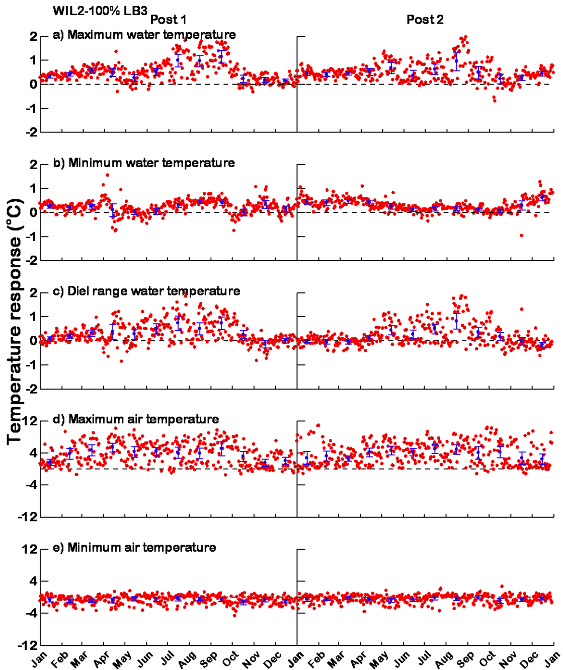
Appendix Figure 7-C-3. Water temperature and air temperature response at site WIL2-100%, location LB3. Red dots are the daily temperature response (TR). Blue dots and error bars are the mean monthly temperature response (MMTR) with 95% confidence intervals (CI).
