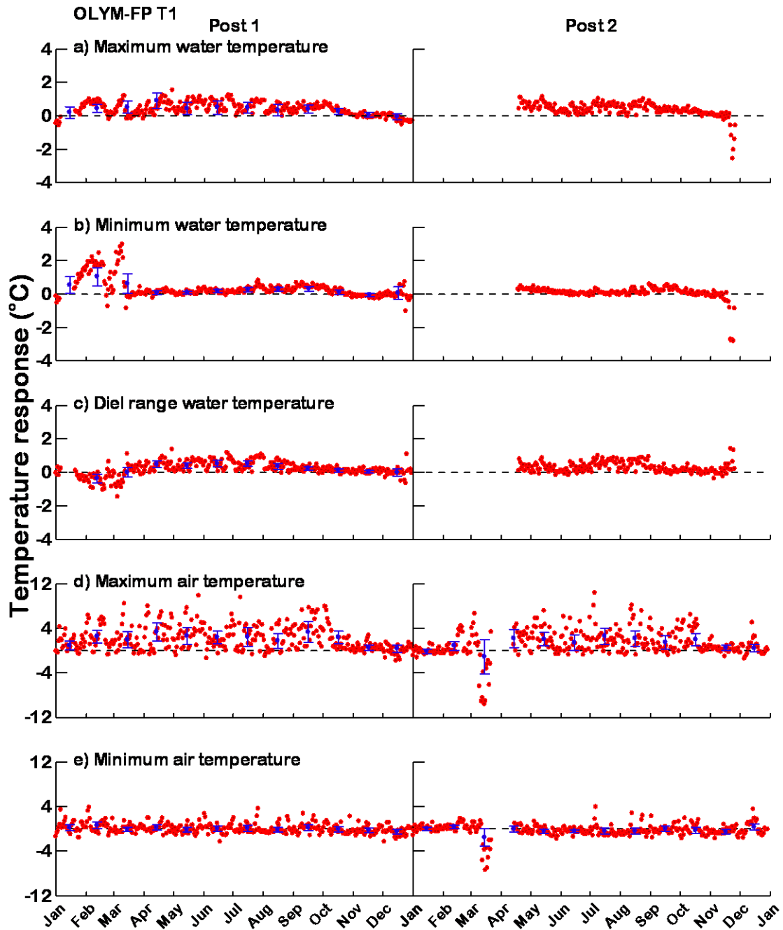
Appendix Figure 7-C-5. Water temperature and air temperature response at site OLYM-FP, location T1. Red dots are the daily temperature response (TR), Blue dots and error bars are the mean monthly temperature response (MMTR) with 95% confidence intervals (CI).
