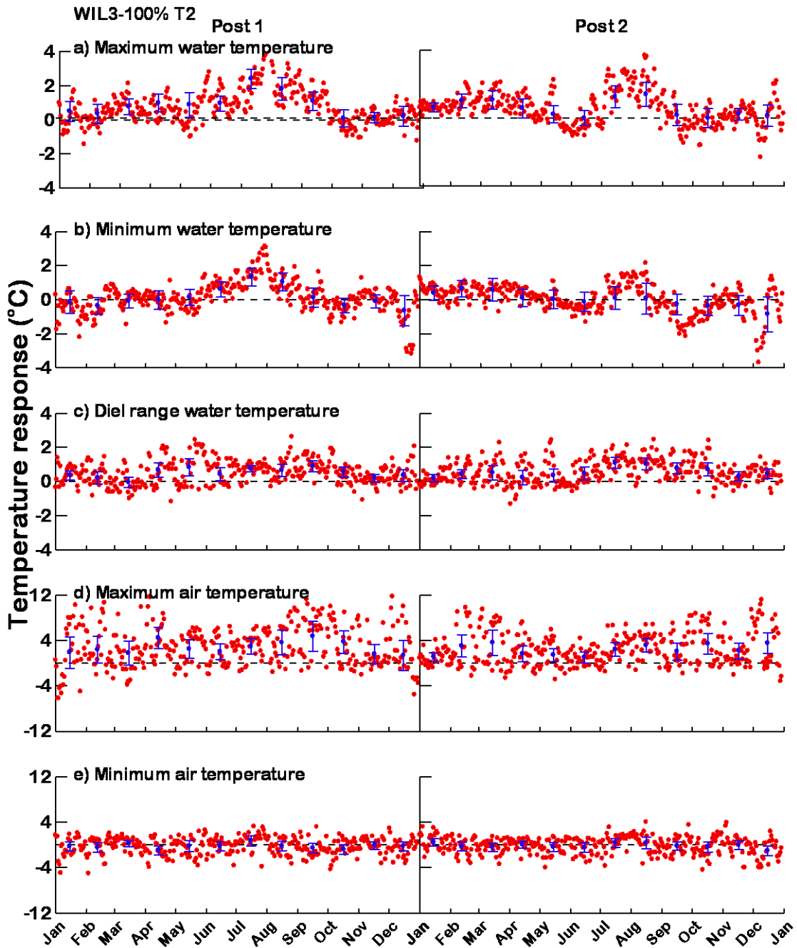
Appendix Figure 7-C-4. Water temperature and air temperature response at site WIL3-100%, location T2. Red dots are the daily temperature response (TR). Blue dots and error bars are the mean monthly temperature response (MMTR) with 95% confidence intervals (CI).
