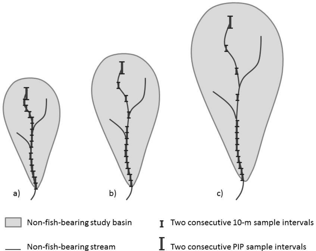
Figure 11-2. Sampling schematic for the (a) smallest (<300 m mainstem length), (b) moderate (300–800 m mainstem length), and (c) largest (>800 m mainstem length) sites.
