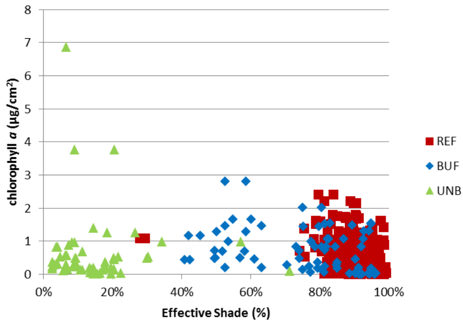
Figure 13-10. Relationship between effective shade (%) and chlorophyll a ( \mu\text{g}/\text{cm}^2 ) for each tile, by buffer (REF = reference, BUF = buffered, UNB = unbuffered).
