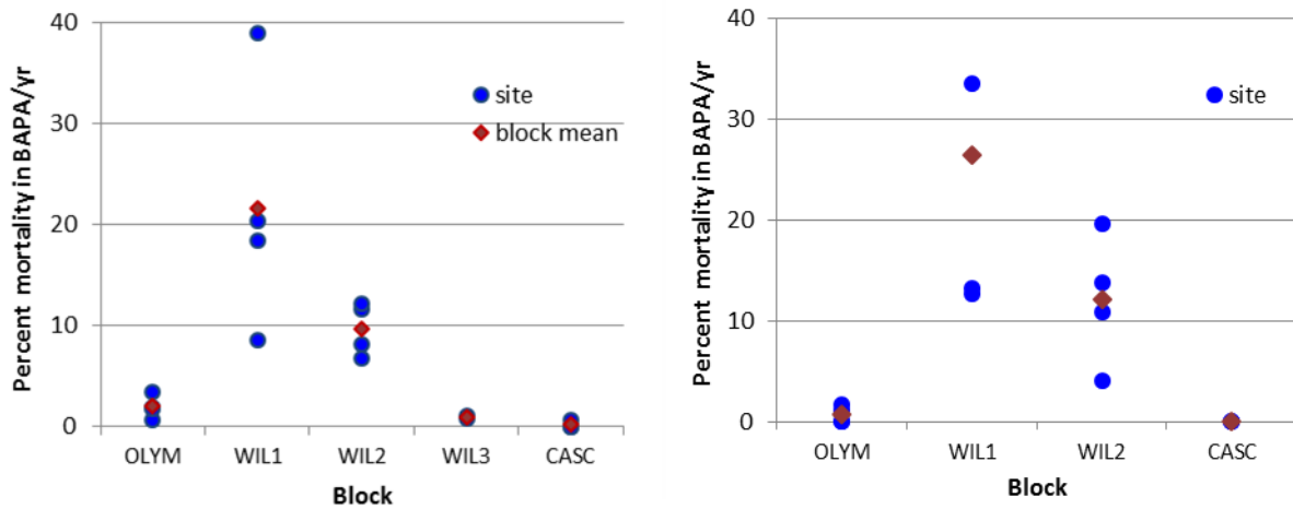
Figure 5-3. Pre-harvest mortality rates (% of basal area/yr) for RMZs (left panel) and PIPs (right panel) by block. Values are site means.
