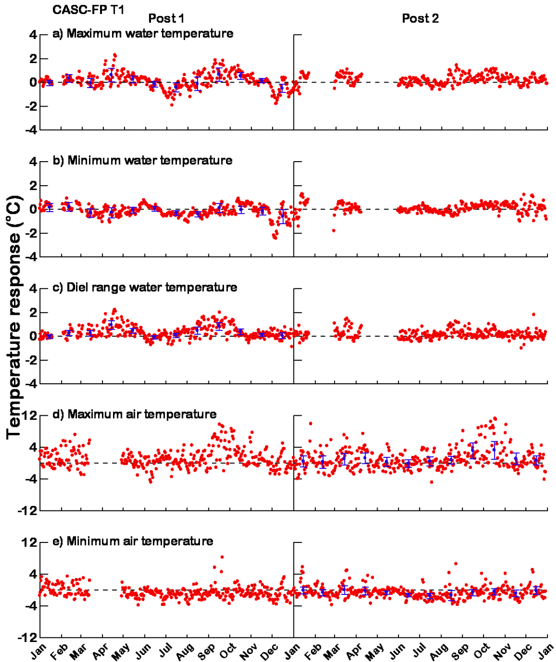
Appendix Figure 7-C-7. Water temperature and air temperature response at site CASC-FP, location T1. Red dots are the daily temperature response (TR). Blue dots and error bars are the mean monthly temperature response (MMTR) with 95% confidence intervals (CI).
