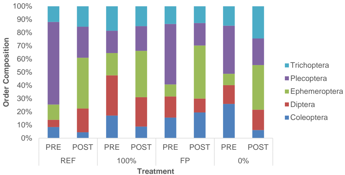
Figure 14-9. Composition of macroinvertebrate export in biomass per day ( \text{mg day}^{-1} ) from the Type N Study treatments by order and treatment period. REF = reference; 100% = 100% treatment; FP = Forest Practices treatment; 0% = 0% treatment; PRE = pre-harvest period; POST = post-harvest period.
