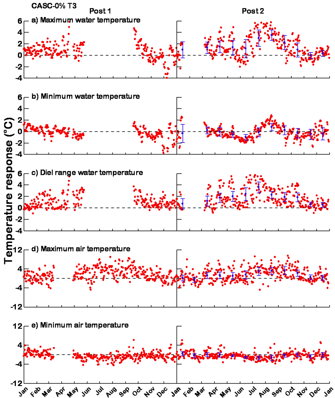
Appendix Figure 7-C-11. Water temperature and air temperature response at site CASC-0%, location T3. Red dots are the daily temperature response (TR). Blue dots and error bars are the mean monthly temperature response (MMTR) with 95% confidence intervals (CI).
