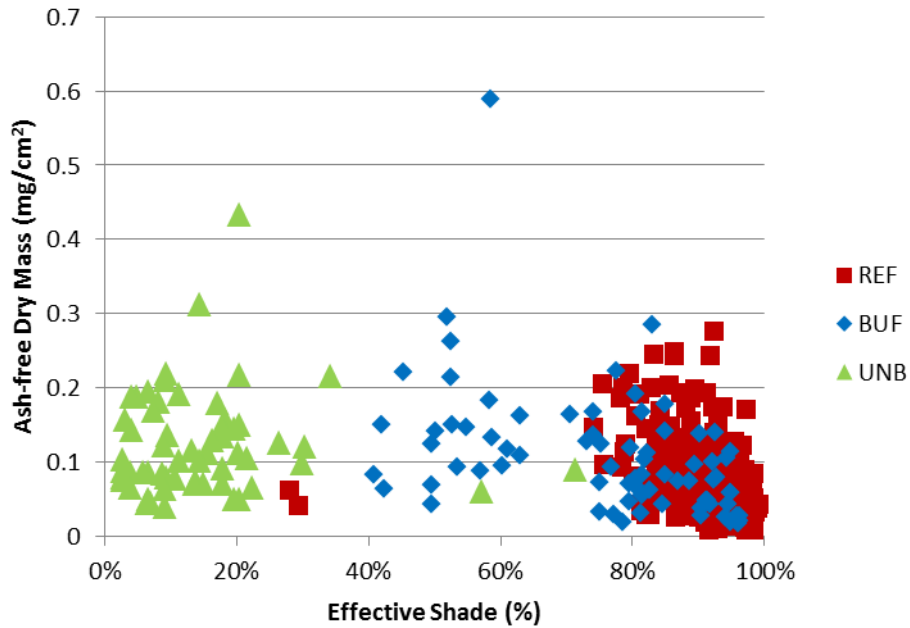
Figure 13-9. Relationship between effective shade (%) and ash-free dry mass ( \text{mg}/\text{cm}^2 ) for each tile, by buffer (REF = reference, BUF = buffered, UNB = unbuffered).
