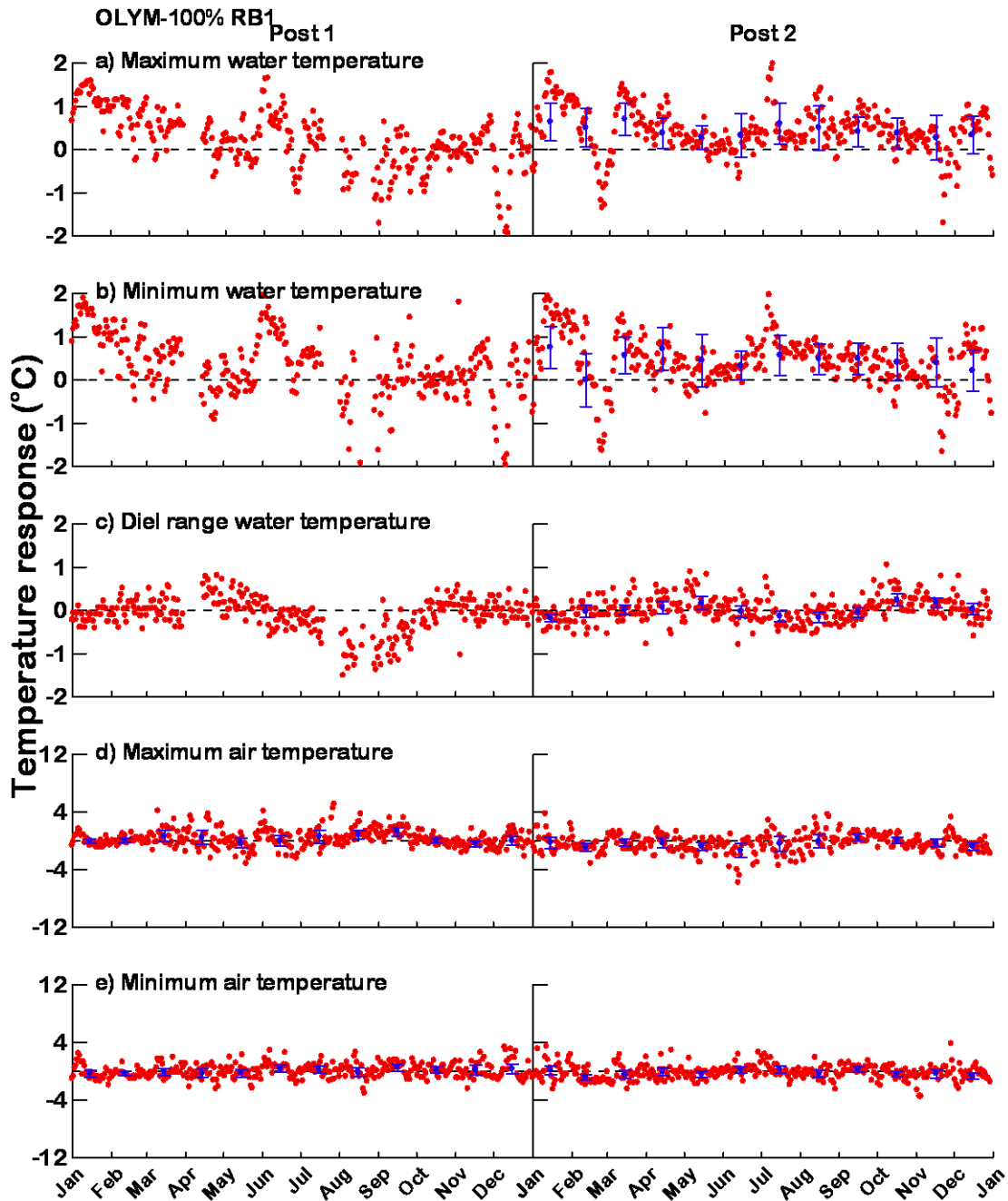
Appendix Figure 7-C-1. Water temperature and air temperature response at site OLYM-100%, location RB1. Red dots are the daily temperature response (TR). Blue dots and error bars are the mean monthly temperature response (MMTR) with 95% confidence intervals (CI).
