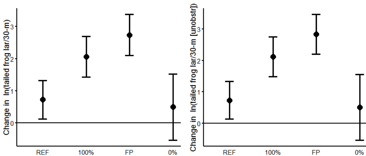
Figure 15-12. The within-treatment change for the natural log (ln) of stream network-wide larval Coastal Tailed Frog density (animals/30 m), i.e., [ln(post) – ln(pre)], and 95% confidence interval (CI) estimated with light-touch sampling adjusted for detection, including (left panel) and excluding (right panel) obstructed reaches.
