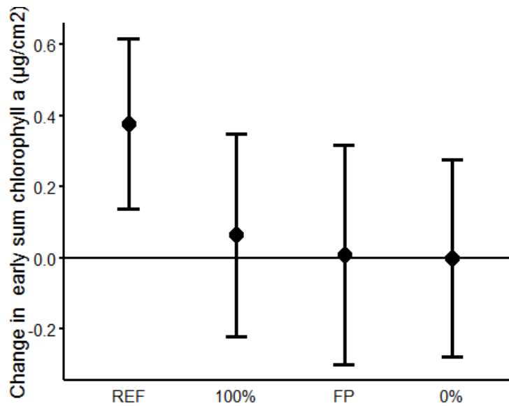
Figure 13-5. The within-treatment change and 95% confidence intervals (CI) for chlorophyll a ( \mu\text{g}/\text{cm}^2 ) in the early summer season, i.e., (post – pre).
