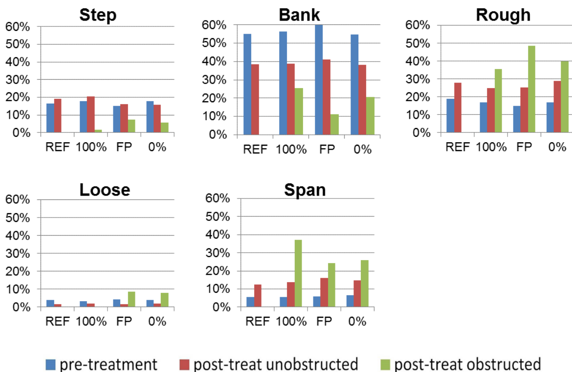
Figure 6-20. Percent of LW contributing to instream function in the pre-harvest period, and stream reaches unobstructed and obstructed by logging debris and windthrow in the post-harvest period, by treatment. Note the absence of obstructed reaches in references.
