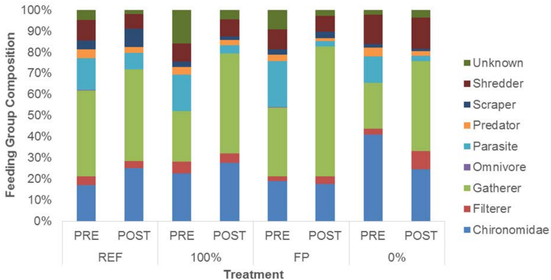
Figure 14-6. Composition of macroinvertebrate export in numbers per day ( \# \text{ day}^{-1} ) from the Type N Study treatments by functional feeding group and treatment period. REF = reference; 100% = 100% treatment; FP = Forest Practices treatment; 0% = 0% treatment; PRE = pre-harvest period; POST = post-harvest period.
