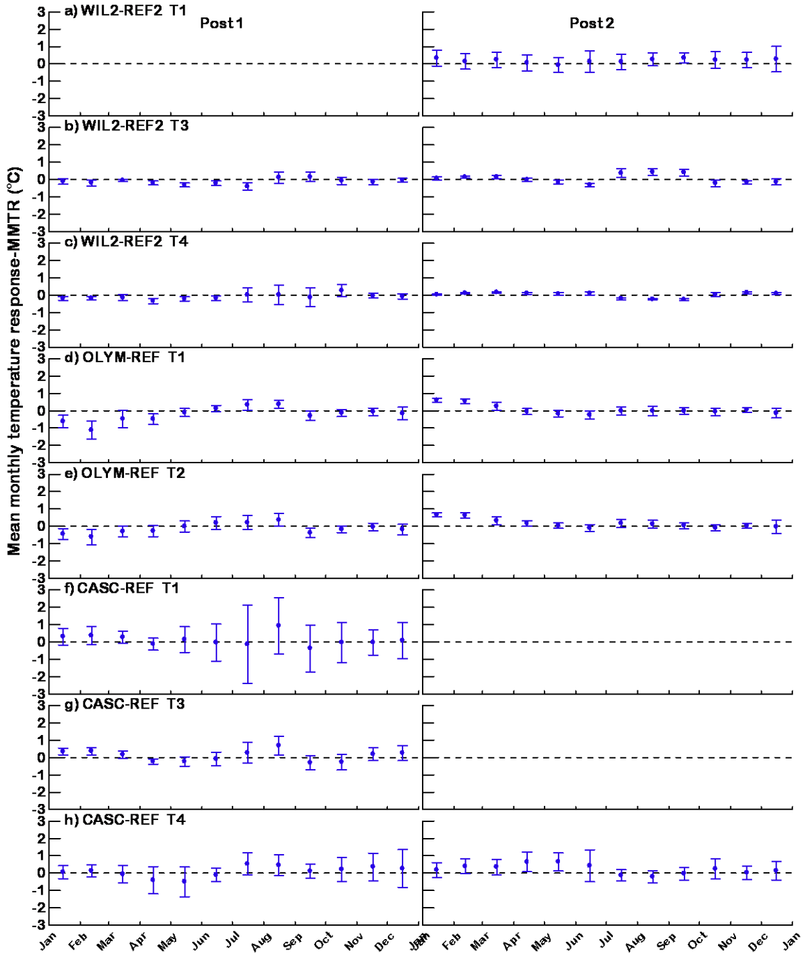
Figure 7-5. Mean monthly temperature response (MMTR) for maximum daily temperature and 95% confidence intervals (CI) calculated from reference-to-reference comparisons for locations in WIL2-REF2 (a-c), OLYM-REF (d-e) and CASC-REF (f-h). We did not calculate MMTR for years with less than 300 consecutive days, or months with less than 20 days, of data.
