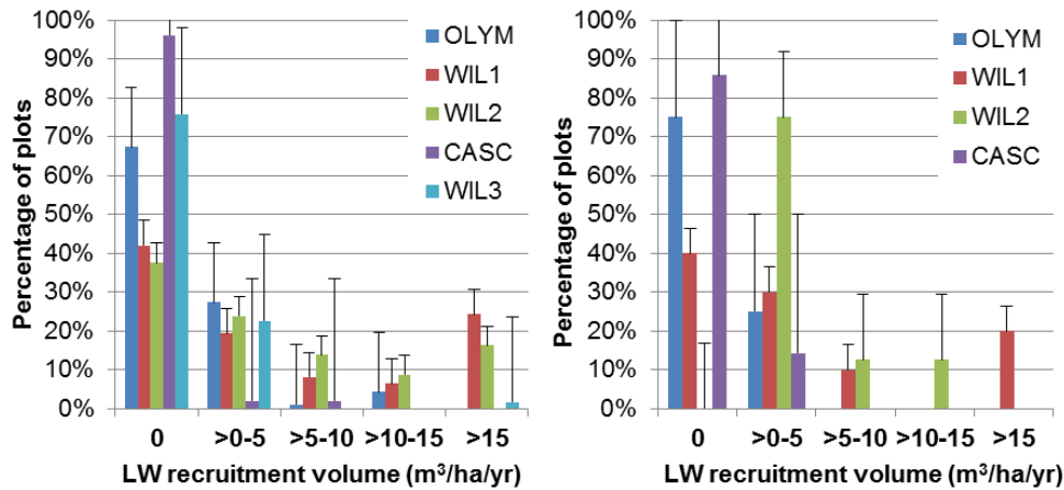
Figure 6-9. Distribution of pre-harvest LW recruitment volume for RMZ (left panel) and PIP plots (right panel) by block.
