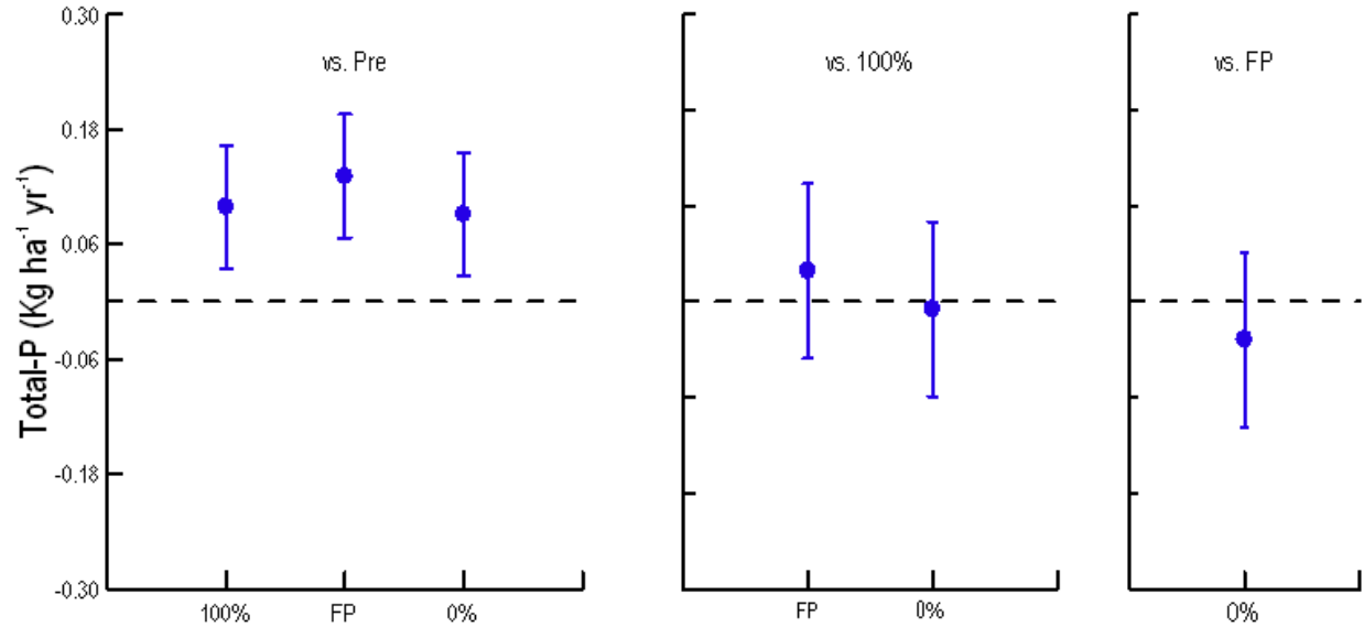
Figure 9-9. Results of the test of the six hypotheses for total-P export. The left panel shows the mean change in export (and 95% confidence intervals) post-harvest in each treatment, hypotheses a), b), and c). The right panel compares the change in export among the three treatments, hypotheses d), e), and f). The horizontal dashed line equals no change. Confidence intervals that do not cross the dashed line indicate the hypothesis is rejected at P < 0.05 .
