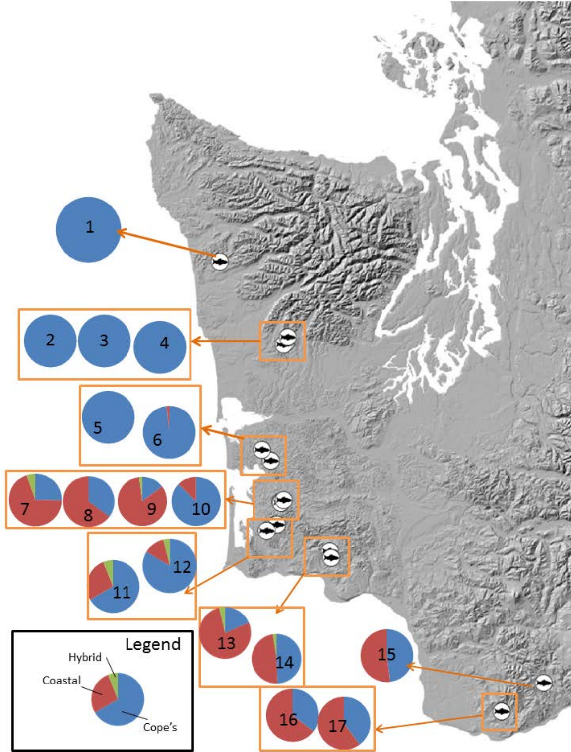
Appendix Figure 15-B-1. Distribution of giant salamanders (Cope's, Coastal and hybrids) across 17 study sites (2006–2011). Sample size and proportion of each species for numbered sites are presented in Appendix Table 15-B-1 .
