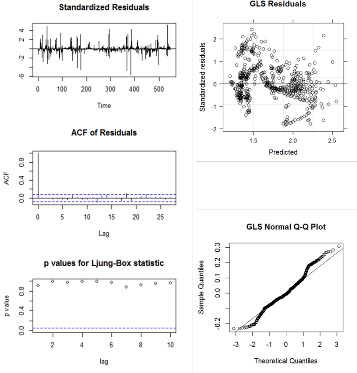
Figure 8-4. GLS regression diagnostic plot for the analysis of discharge in the WIL1-0% using the combined ARMA model. (Equation 8-6). The plots on the left are the same as shown in Figure 8-2 and confirm that the residual autocorrelation has been removed, the top right shows that there is no pattern in the residuals (e.g., no heteroscedasticity), and the bottom right shows that the residuals are approximately normally distributed (e.g., \varepsilon \sim N(0, \sigma^2, I) ).
