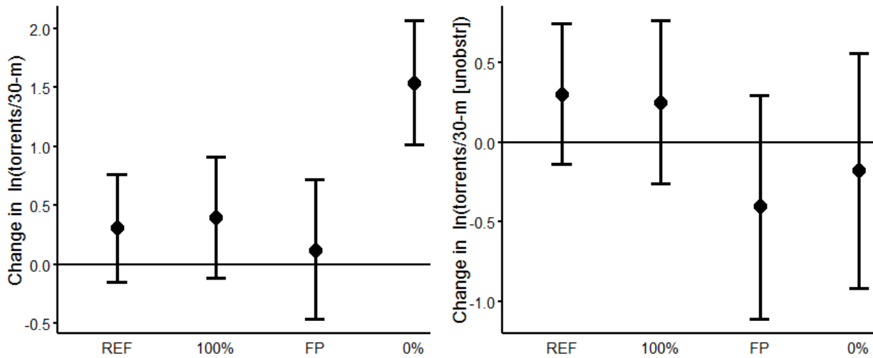
Figure 15-14. The within-treatment change for the natural log (ln) of stream network-wide torrent salamander linear density (animals/30 m), i.e., [ln(post) – ln(pre)], and 95% confidence interval (CI) estimated with light-touch sampling adjusted for detection, including (left panel) and excluding (right panel) obstructed reaches.
