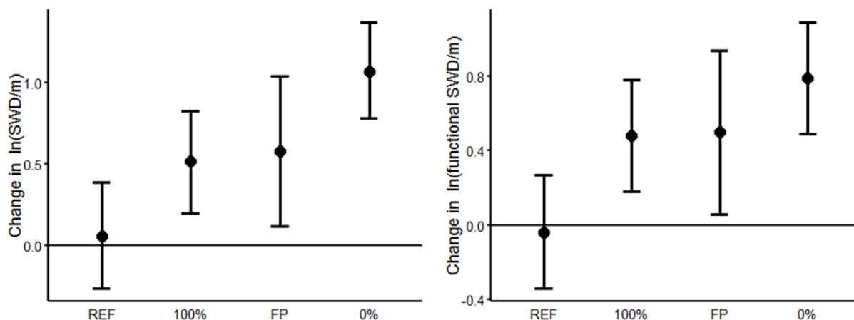
Figure 6-13. The within-treatment change and 95% confidence intervals (CI) for the natural log (ln) of the number of SW pieces per meter (left panel) and number of functional SW pieces per meter (right panel), i.e., [\ln(\text{post}) - \ln(\text{pre})] .
