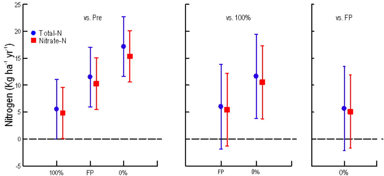
Figure 9-8. Results of the test of the six hypotheses for total-N and nitrate-N export. The left panel shows the mean change in export (and 95% confidence intervals) post-harvest in each treatment, hypotheses a), b), and c). The right panel compares the change in export among the three treatments, hypotheses d), e), and f). The horizontal dashed line equals no change. Confidence intervals that do not cross the dashed line indicate the hypothesis is rejected at P < 0.05 .
