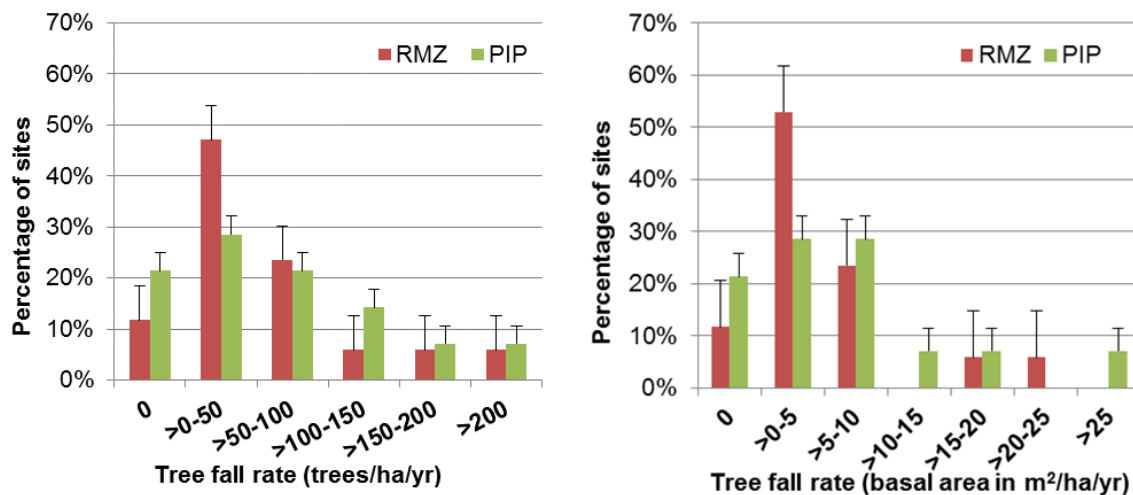
Figure 6-2. Percentage of sites by mean tree fall rate in trees/hectare/yr (left panel) and basal area in m 2 /hectare/yr (right panel) for RMZs and PIPs in the pre-harvest period.
