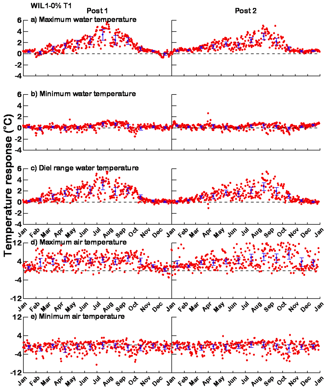
Appendix Figure 7-C-9. Water temperature and air temperature response at site WIL1-0%, location T1. Red dots are the daily temperature response (TR). Blue dots and error bars are the mean monthly temperature response (MMTR) with 95% confidence intervals (CI).
