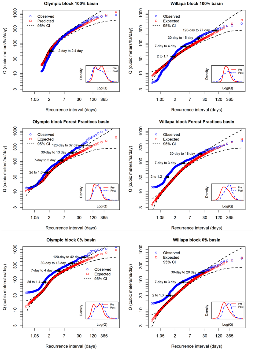
Figure 8-9. Discharge frequency curves for the two years post-harvest (730 days). Inset graphs show the distribution of log-transformed discharge, while the larger graphs shows discharge magnitude on a logarithmic axis as a function of recurrence interval (RI). Shifts in the frequency distribution that extend beyond the 95% confidence interval (CI) are displayed with arrows for 2, 7, 30, and 120-day events.
