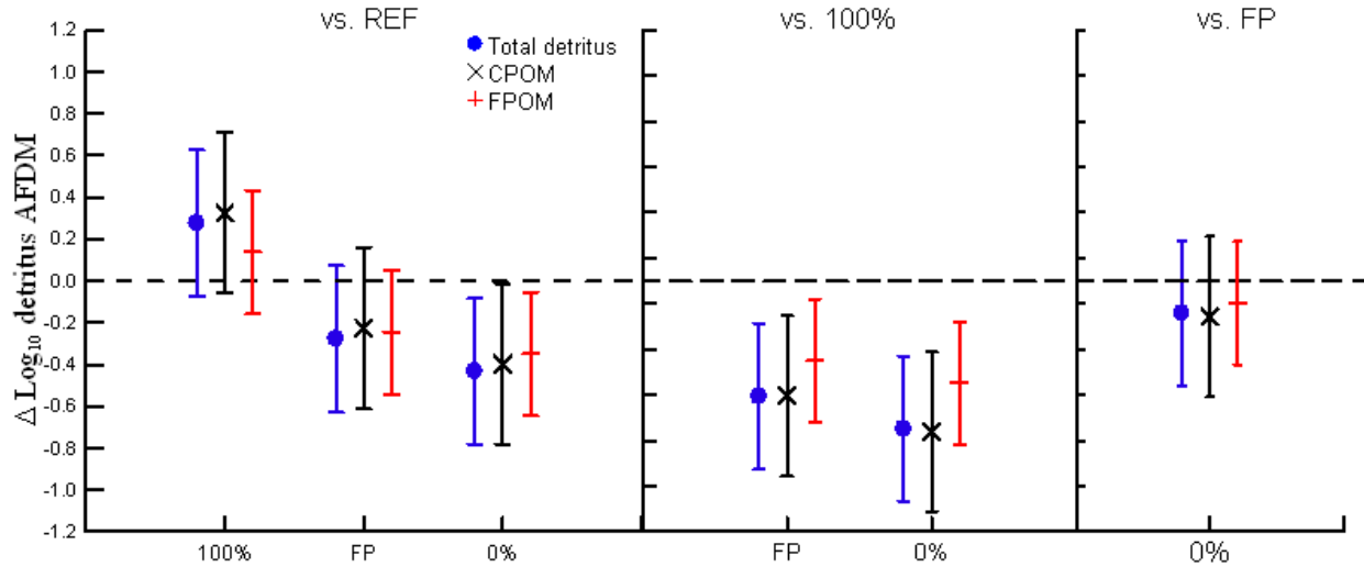
Figure 12-7. Results of the test of the six hypotheses for total, coarse particulate organic matter (CPOM; >1 mm), and fine particulate organic matter (FPOM; <1 mm) detritus export. The left panel shows the change in detritus export post-harvest in each treatment relative to the reference. The right two panels compare the change in detritus export among the three treatments. The error bars are 95% confidence intervals (CI). The horizontal dashed line equals zero (no change). Confidence intervals that do not cross the dashed line indicate the hypothesis is rejected at P < 0.05 .
