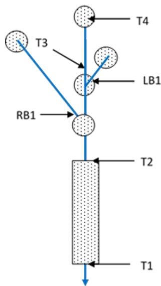
Figure 7-1. Conceptual layout of Forest Practices riparian buffers and temperature monitoring locations.
