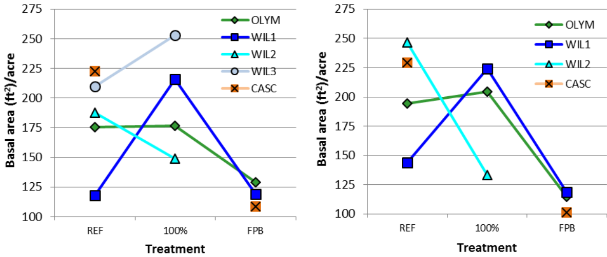
Figure 5-10. Basal area (ft 2 /ac) the second summer post-harvest by experimental treatment for RMZs (left panel) and PIPs (right panel).
