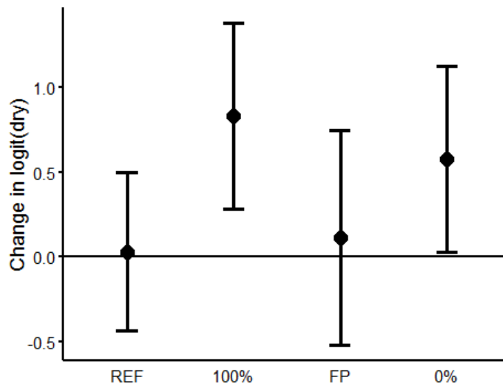
Figure 11-6. The within-treatment change and 95% confidence interval (CI) for the logit-transformed proportion of the stream characterized as dry, i.e., [logit(post) – logit(pre)].
