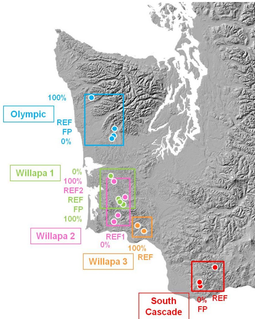
Figure 12-1. Distribution of the Type N study sites and treatments. Study sites are blocked and based on geography. Litterfall and detritus samples were collected from the Olympic (color-coded blue) and Willapa 1 (color-coded green) blocks. REF = reference; 100% = 100% treatment; FP = Forest Practices treatment; 0% = 0% treatment.
