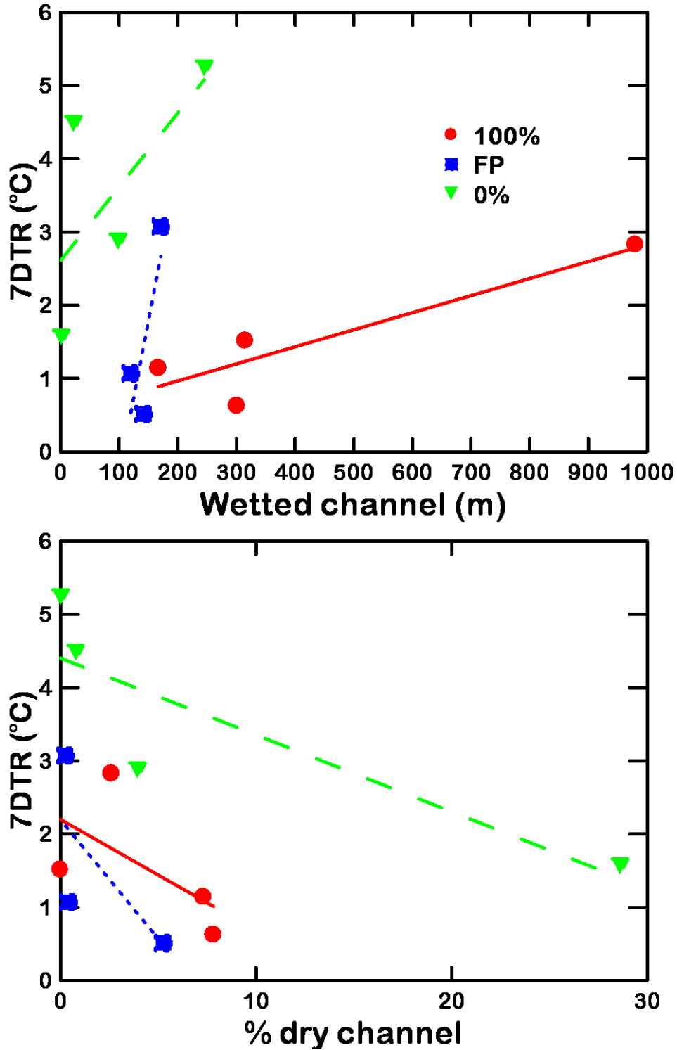
Figure 7-13. Change in 7DTR plotted against length of wetted channel above the monitoring location (top panel) and percent of the perennial Type N channel that had no summer surface flow (bottom panel). The temperature effect data are from the first post-harvest year. The % dry channel data are an average of surveys taken in the summers of 2006 and 2010.
