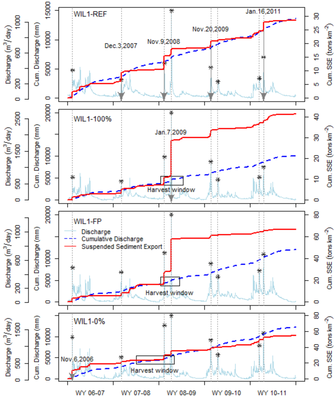
Figure 10-3. Discharge, cumulative discharge and cumulative SSE in the four sites in the Willapa 1 block. Peak daily discharge denoted by asterisk. Vertical dashed lines correspond with storms that resulted in major sediment export at one or more sites, and arrows are associated with dates for an event.
