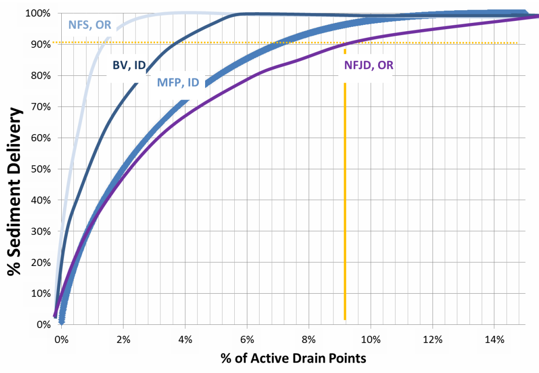
Figure 1. Pareto analysis of sediment delivery from four GRAIP watershed surveys (Black et al. 2013).
