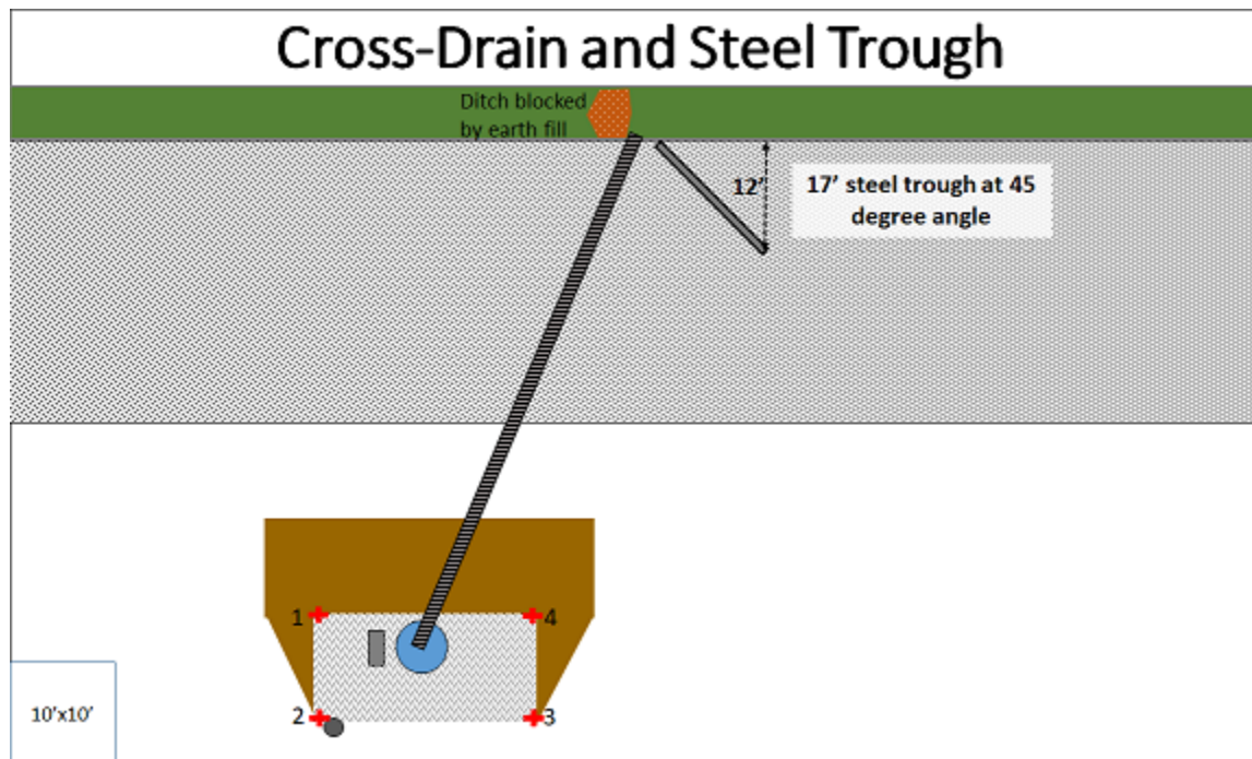
Figure 4. Configuration of bottom end of an 80-meter segment. Ditch (in green) is blocked below cross-drain culvert by earthen headwall. Steel trough is 17-feet-long and placed on a 45-degree angle up the road to capture 12 feet of the tread and drain into the ditch line 1 foot above the cross-drain culvert inlet. The cross-drain culvert is on a strong skew to create a 5% gradient in the pipe and it extends several feet beyond the edge of the tread (in gray) to a platform that holds equipment.
