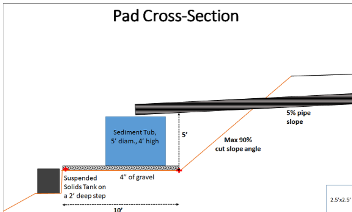
Figure 6. Cross-sectional view of the platform components.
