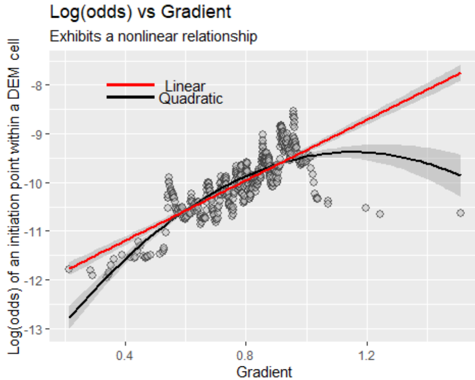
Figure 4: Log(odds) of landslide density versus gradient
