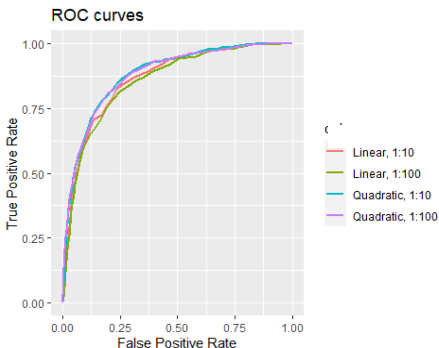
Figure 17: ROC curves
