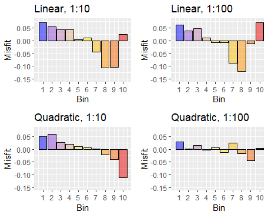
Figure 16: Misfit of modeled landslide proportions within each 10% bin.
