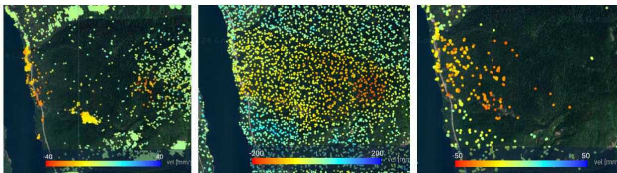
Figure 5-9. Spatial displacement data coverage for a large rock slide along the Columbia River in British Columbia for (left to right) Sentinel-1 C-Band, ALOS-2 Fine L-Band, ALOS-2 ScanSAR L-Band data.
