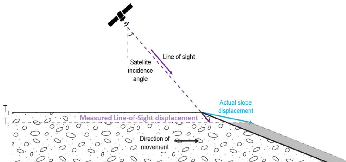
Figure 5-8. Simplified schematic diagram illustrating the line-of-sight measurement of the true displacement.
