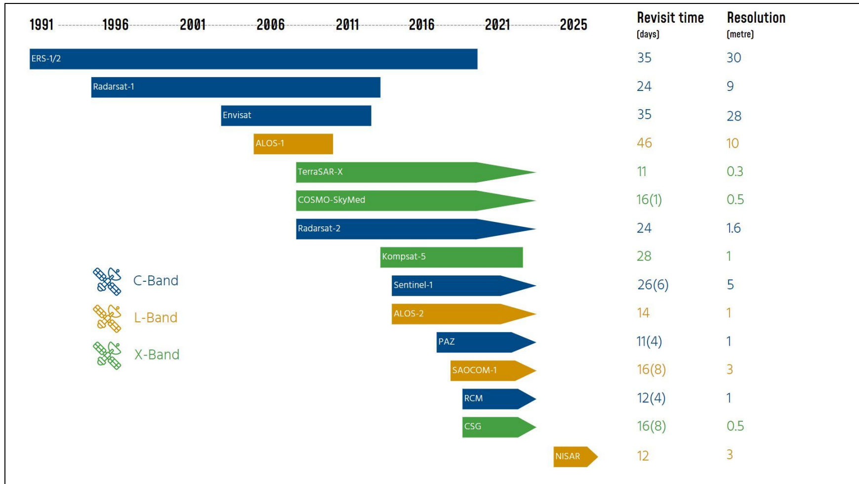
Figure 3-6. Overview of the historic, current, and upcoming SAR satellites launched by various international space agencies. A pointed right-end on the bars shown indicates ongoing data collection, whereas a square end indicates a cessation in satellite acquisition.
