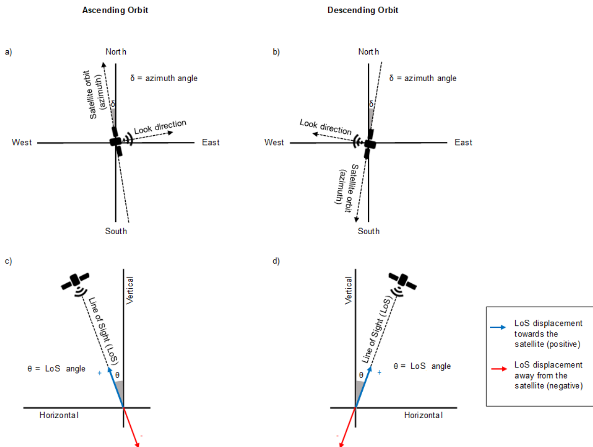
Figure 5-7. Satellite acquisition geometries and sign of the measured displacement relative to the satellite for the ascending orbit (“a” and “c”) and descending orbit (“b” and “d”).
